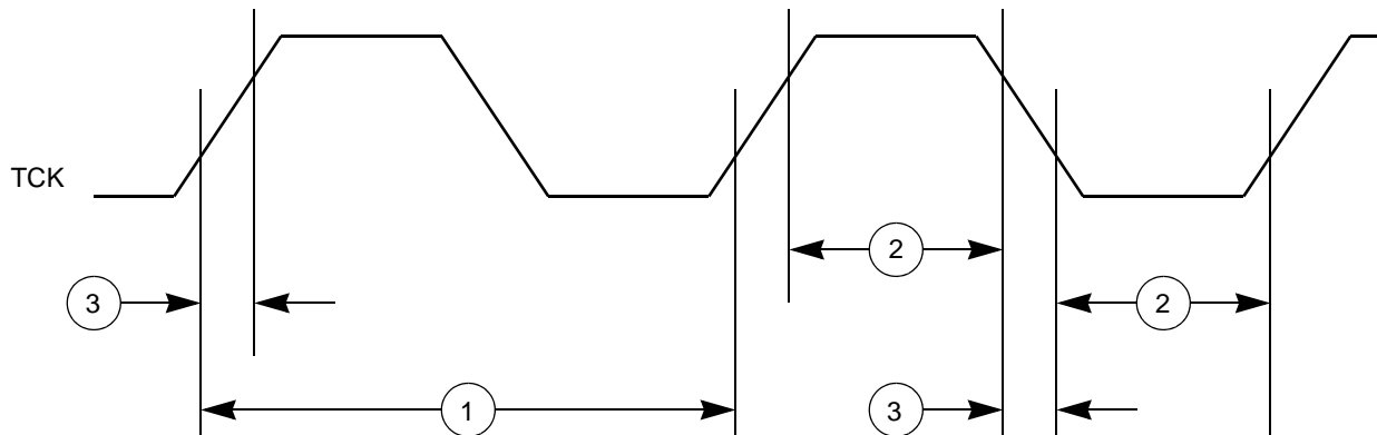
Figure 8. JTAG Test Clock Input Timing
